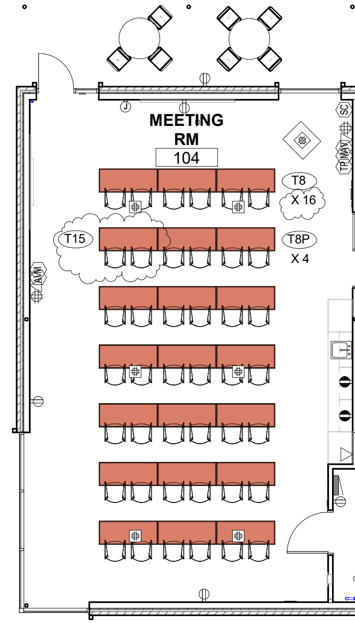
2 MEETING ROOM TABLE LAYOUT F1.00 1/8" = 1'-0"
