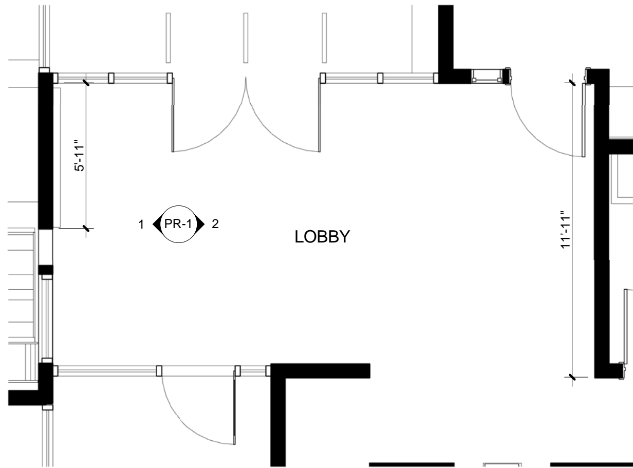
3 HISTORY WALL- FLOOR PLAN 1/4" = 1'-0"
