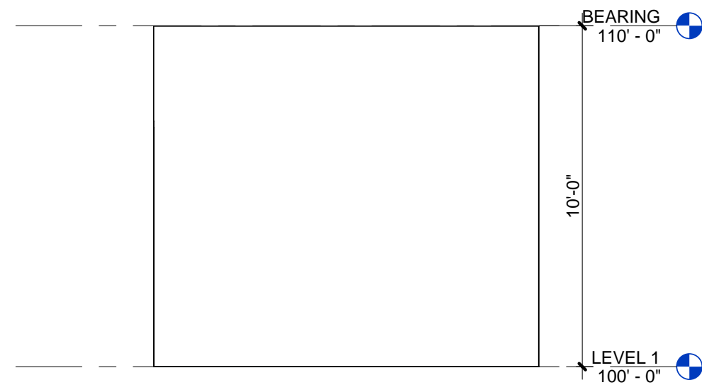
2 EAST WALL 1/4" = 1'-0"
